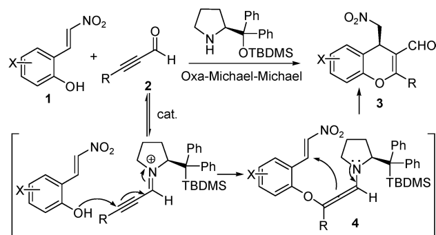
Scheme 1. Alkynals Participating in Enantioselective Cascade Oxa-Michael–Michael and –Aldol Reactions Promoted by a Chiral Secondary Amine Involving a Novel Iminium-allenamine Activation Mode
