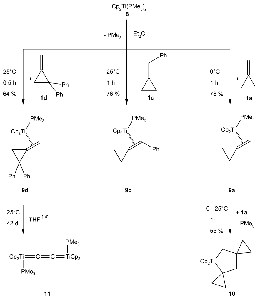
Scheme 3. Reactions of \text{Cp}_2\text{Ti}(\text{PMe}_3)_2 ( 8 ) methylenecyclopropane 1a , 1c and 1d .
