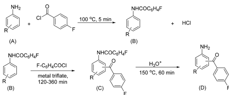
Scheme 2. Synthesis of aminobenzophenone derivatives via Friedel–Crafts benzoylation
