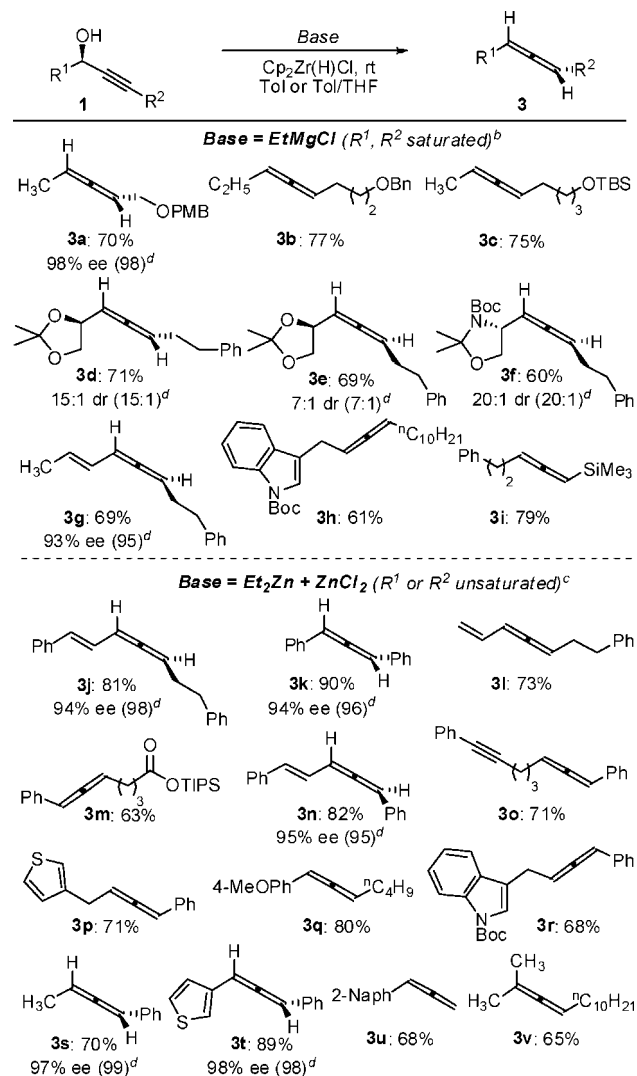
Figure 1. Synthesis of allenes from propargylic alcohols. a Isolated yields. Allenes are drawn such that the original alkyne substituent ( R^2 ) is on the right. See Supporting Information for experimental details. b 1 equiv of EtMgCl; 0.2 M in toluene; 1.1 equiv of Cp_2ZrHCl . c 0.5 equiv each of Et 2 Zn, ZnCl 2 ; 0.2 M in toluene/THF 30:1; 1.6 equiv of Cp_2ZrHCl . d Values in parentheses represent ee or dr of starting material.
