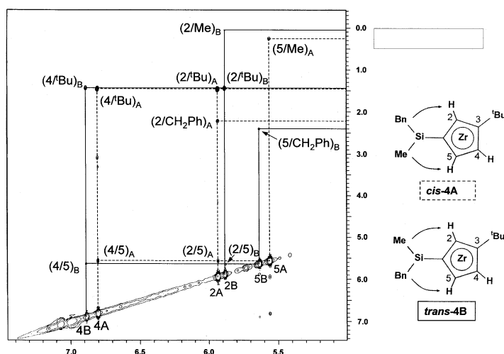
Fig. 2. ^1\text{H} -ROESY spectrum of the ansa -zirconocene product mixture containing 4A and 4B , in \text{C}_6\text{D}_6 solution. Broken lines correlate signals of isomer 4A , solid lines those of isomer 4B .
