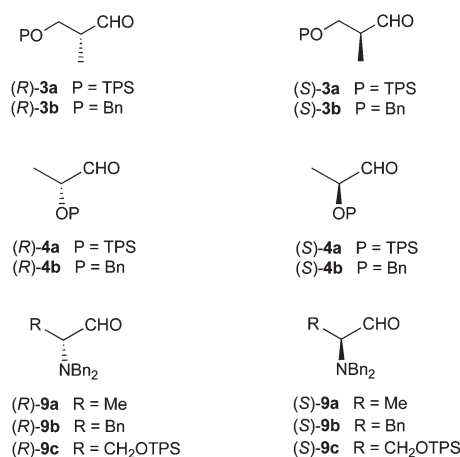
Fig. 1 \alpha -Chiral aldehydes used in this study (TPS = tert -butylphenylsilyl).
