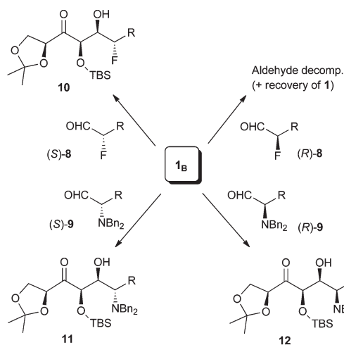
Scheme 2 Aldol additions of enolate 1 B to aldehydes ( R )/( S )-3, ( R )/( S )-4, ( R )/( S )-8 and ( R )/( S )-9 (Bn = benzyl).
