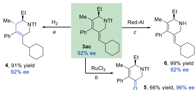
Scheme 4. Derivatization of the Chiral Products a
