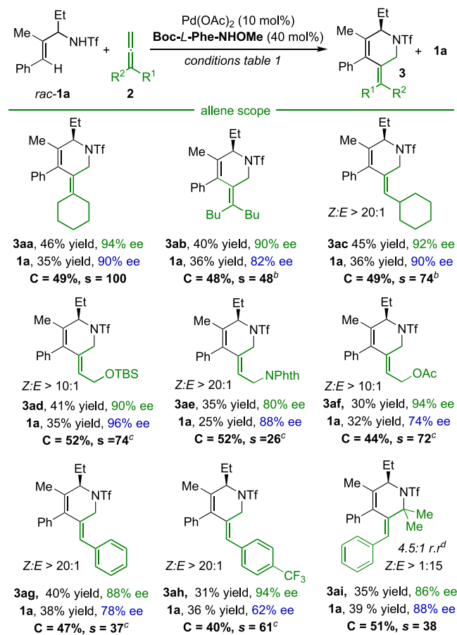
Scheme 2. Scope of the Formal (4+2) Cycloaddition of Allyl-trifluoromethylamides and Allenes a
