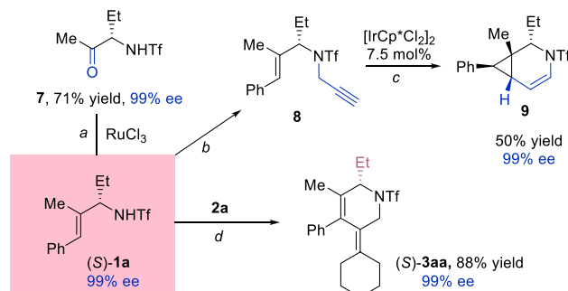
Scheme 5. Derivatization of the Chiral Allylamide Starting Materials a
