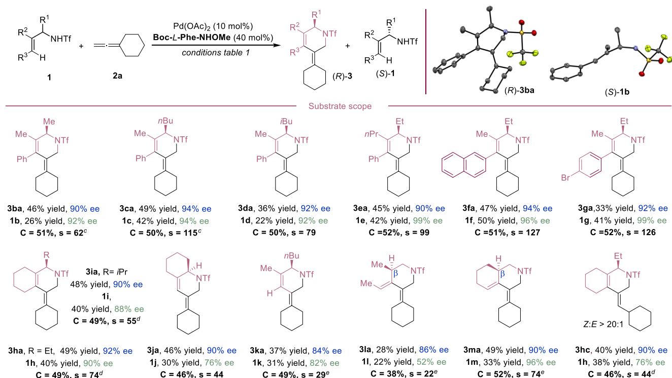
Scheme 3. Scope of the Formal (4+2) Cycloaddition of Allyltriflamides and Allenes a,b
