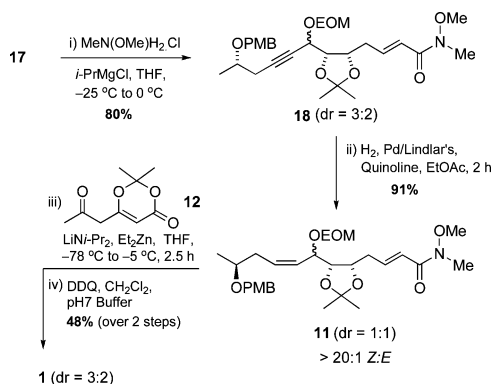
Scheme 4. Synthesis of Weinreb Amide 11 and Diketo-dioxinone 1
