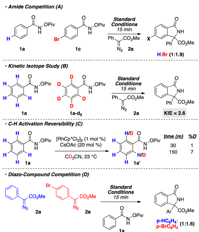
Scheme 1. Mechanistic Experiments
