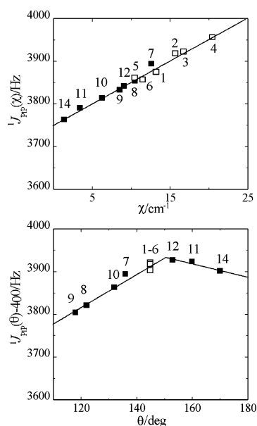
Figure 10. Electronic profile (upper plot) and steric profile (lower plot) for the ^1J_{\text{PtP}} values of [\text{PtMe}(\text{Me}_2\text{-phen})(\text{PR}_3)]^+ complexes.
