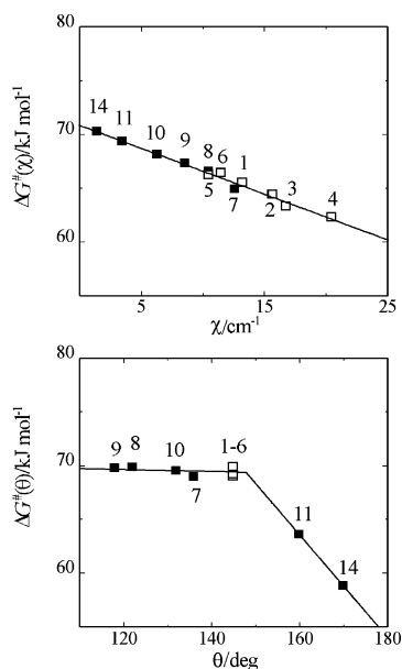
Figure 9. Electronic profile (upper plot) and steric profile (lower plot) for the free activation energy of the fluxional motion of \text{Me}_2\text{-phen} in [\text{PtMe}(\text{Me}_2\text{-phen})(\text{PR}_3)]^+ . Open squares refer to complexes containing triaryl \text{P}(4\text{-XC}_6\text{H}_4)_3 phosphanes.
