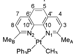
Chart 1. Structural Formula of Complexes with Atomic Numbering
