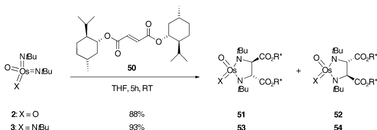
Scheme 11. Diastereoselective diamination of bis[(-)-menthyl] fumarate ( 50 ) [ R^*OH = (-)\text{-menthol} ].
