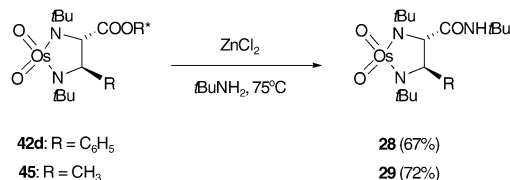
Scheme 10. Functional group transformation of osmaimidazolidines.
