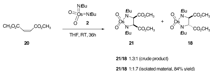
Scheme 4. Diamination of maleic ester 20 .
