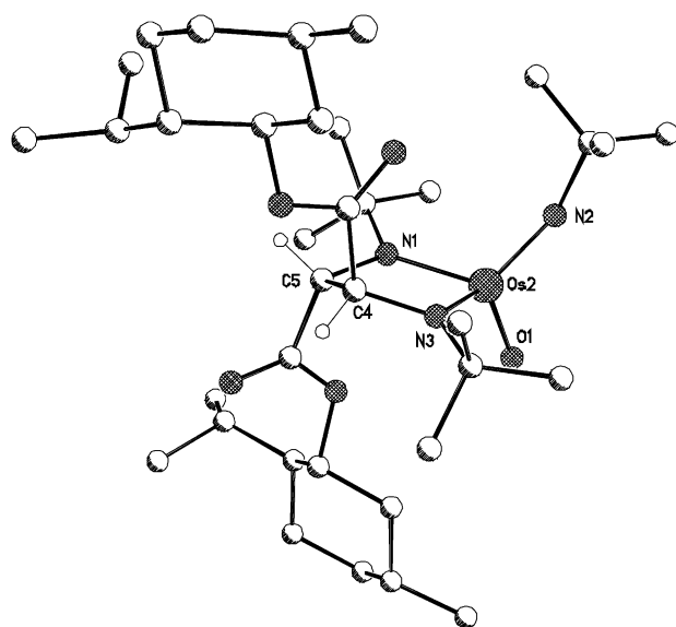
Figure 7. Solid-state structure of major diastereoisomer 53 (except for the stereogenic centres at C4 and C5, hydrogen atoms are omitted). Selected bond lengths [Å] and angles [°]: Os2–O1 1.707(6), Os2–N2 1.727(7), Os2–N3 1.887(8), N1–Os2 1.893(7), N2–Os2–N3 112.5(3), O1–Os2–N1 110.6(3), O1–Os2–N2 115.5(3), N3–Os2–N1 81.9 (3), C36–N2–Os2 157.4(6).
