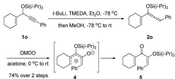
Scheme 3. Rubottom Oxidation of O -Silylated Allenol Ethers
