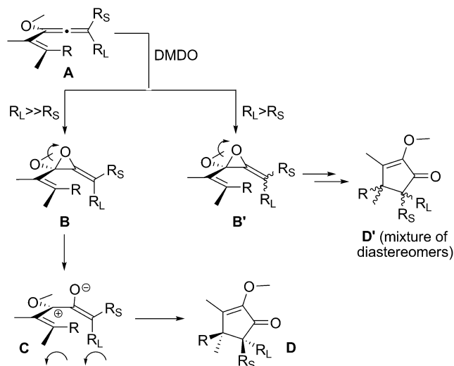
Scheme 5. Proposed Mechanistic Rationale for Observed Diastereochemistry
