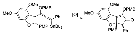
Scheme 1. Oxidation-Initiated Nazarov Cyclization in the Synthesis of (±)-Rocaglamide
