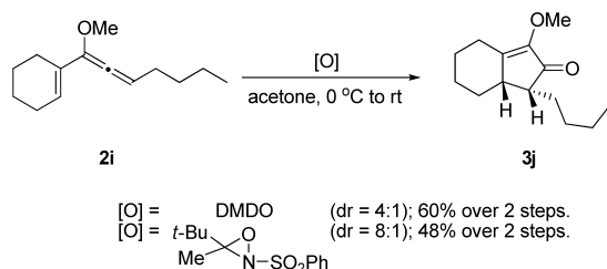
Scheme 4. Cyclization of 2i with Use of a Bulky Oxaziridine
