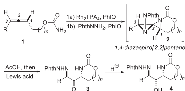
Scheme 1. Bis-aziridination as a Key Step in the Conversion of Allenes to 1,3-Diamino-2-ols via DASP Intermediates
