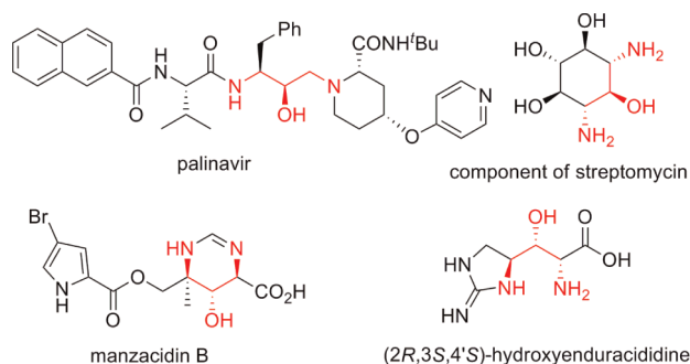
Figure 1. Biologically active 1,3-diamino-2-ols.
