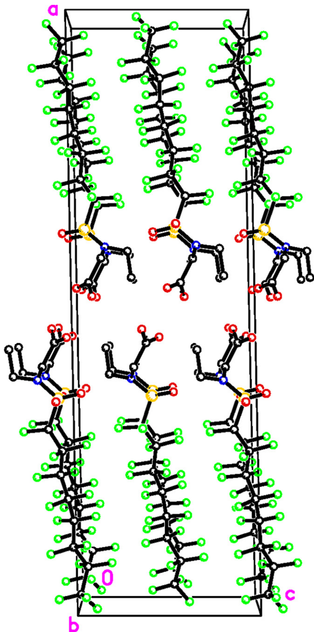
Fig. 6. Packing diagram of 2-(N-ethyl-perfluorooctanesulfonamido) acetic acid ( 12 ), viewed down the b axis, illustrating the bilayers of 12 oriented parallel to the b – c plane. H atoms have been omitted for clarity.
