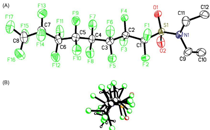
Fig. 2. View of N,N -diethyl-perfluorooctane-1-sulfonamide ( 7e ). (A) Structure of 7e showing the atom-labelling scheme. (B) View of 7e along the carbon backbone to illustrate the helical conformation of the perfluorooctyl chain of the major component in the crystal. Displacement ellipsoids are drawn at the 50% probability level.
