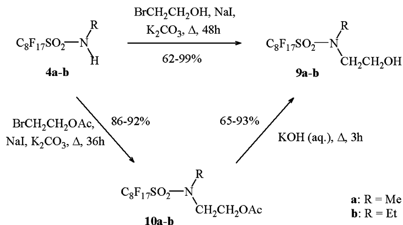
Scheme 2. Synthesis of mono- or N -alkylated perfluorooctanesulfonamidoethanol 9a and 9b .
