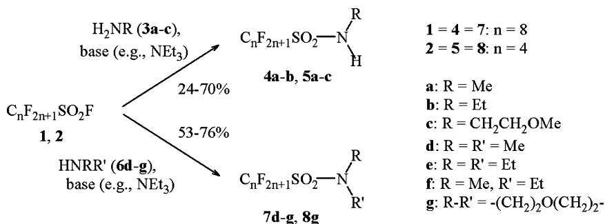
Scheme 1. Synthesis of mono- and dialkylated perfluorooctanesulfonamides.
