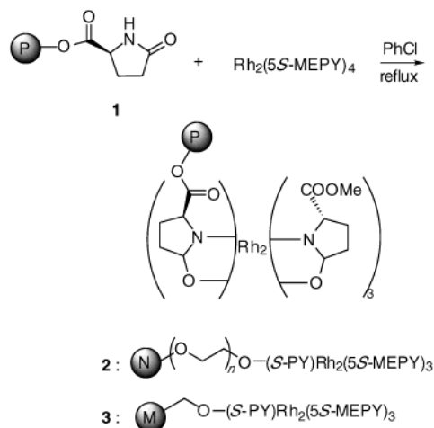
Scheme 1. Preparation of Immobilized Chiral Dirhodium Carboxamides
