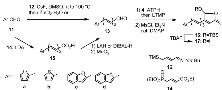
Chart 2. Synthesis of \gamma -Hydroxybutenolides 17a–d
