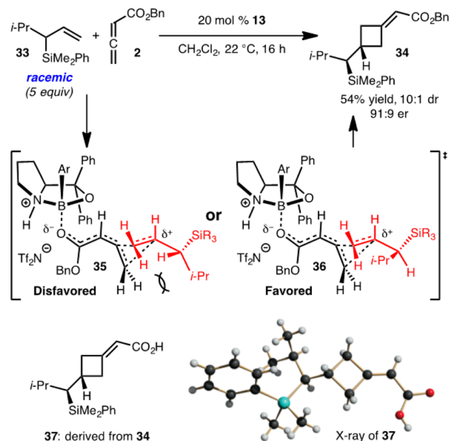
Scheme 7. Kinetic Resolution of Racemic Alkenes
