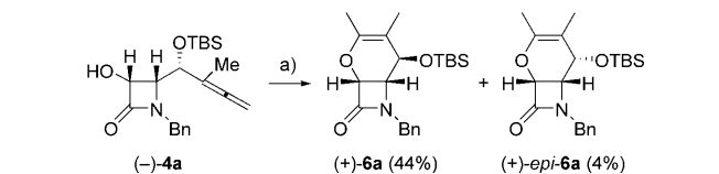
Scheme 1. Lanthanum-promoted preparation of six-membered oxacycles 6a and epi - 6a . a) 5 mol % La[N(SiMe 3 ) 2 ] 3 , toluene, reflux; TBS= tert -butyldimethylsilyl.
