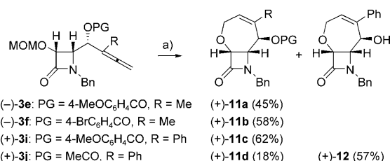
Scheme 5. \text{Au}^{\text{III}} -catalyzed heterocyclization reaction of MOM-protected \gamma -allenol derivatives 3e , 3f , 3i , and 3j . a) \text{AuCl}_3 (5 mol %), \text{CH}_2\text{Cl}_2 , RT.
