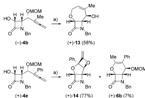
Scheme 6. \text{La}^{\text{III}} -catalyzed heterocyclization reactions of \gamma -allenol derivatives 4b and 4e . a) \text{La}[\text{N}(\text{SiMe}_3)_2]_3 (5 mol %), toluene, reflux.
