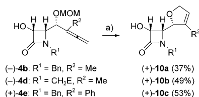
Scheme 4. Gold-catalyzed heterocyclization of \gamma -allenol derivatives 4b , 4d , and 4e . a) \text{AuCl}_3 (5 mol %), \text{CH}_2\text{Cl}_2 , RT; \text{E} = \text{CO}_2\text{Me} .
