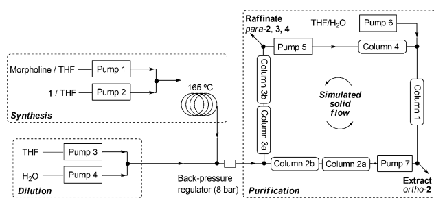
Figure 2. Schematic diagram of the directly coupled system.
