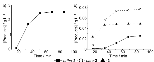
Figure 3. Concentration profiles at the a) extract port in the uncoupled system; b) raffinate port in the uncoupled system.
