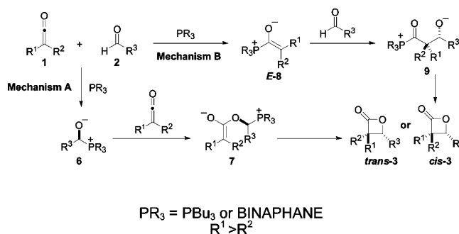
Scheme 2. Postulated Mechanisms A and B for Phosphine-Catalyzed Formal [2 + 2] Cycloaddition of Ketoketenes and Aldehydes
