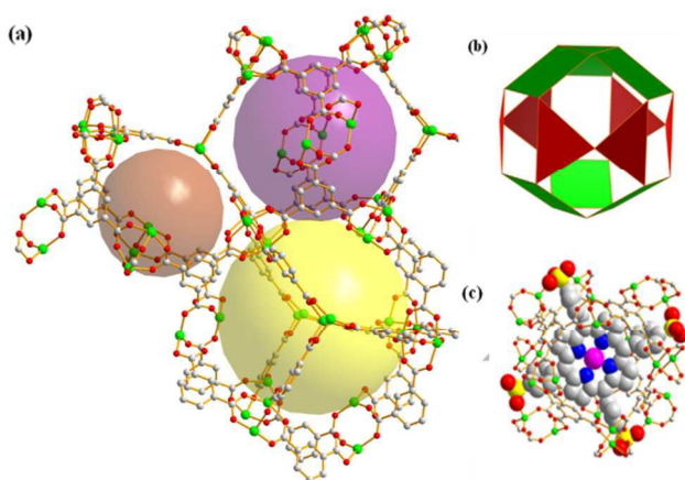
Fig. 1. (a) Three types of polyhedral cages in porphMOM-1 (large cage filled in yellow, middle cage filled in violet and prism filled in brown); (b) large cage comprised of 6 triangular paddlewheel and 6 square paddlewheel moieties; (c) middle cage which contains coordinated FeTPPS moieties (space-filling mode, Zn green, S yellow, N blue, Fe purple).
