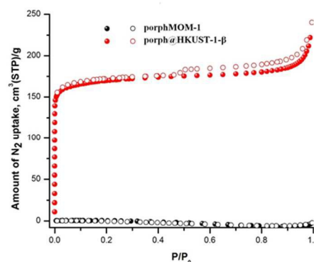
Fig. 3. N 2 sorption isotherms of porphMOM-1 and porph@HKUST-1-β at 77K.
