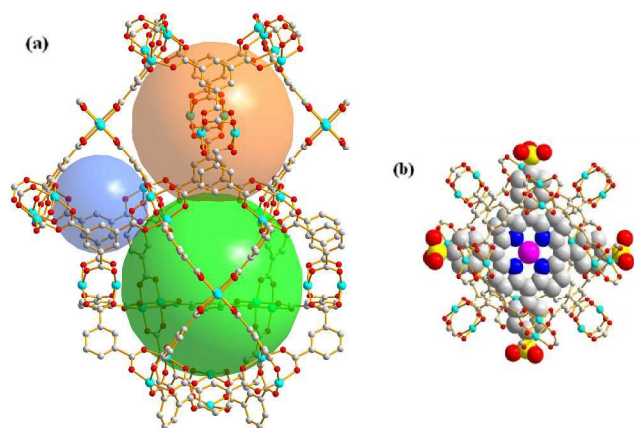
Fig. 2. (a) Three types of polyhedral cages exist in porph@HKUST-1-β (nanoball-2, green, octahemioctahedral cage, orange and tetrahedral cage, blue); (b) octahemioctahedral cage with encapsulated FeTPPS moieties. FeTPPS moieties are highlighted in space-filling mode (Cu cyan, S yellow, N blue, Fe purple).
