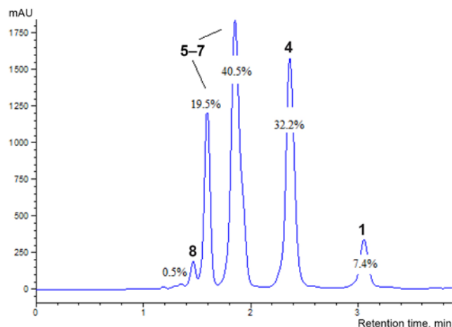
Figure 1. The HPLC result of the aqueous extract after N -methylenation in the synthesis of compound 3d .
