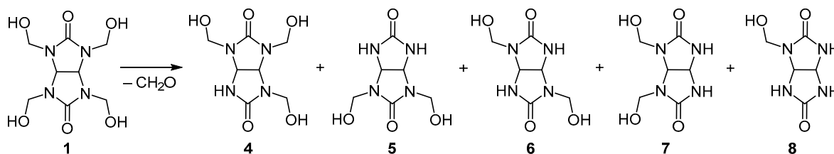
Scheme 2. Dehydroxymethylation products of THGU ( 1 )
