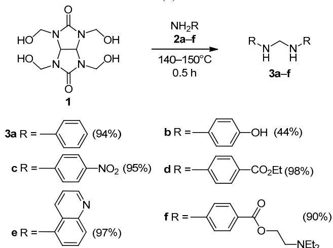
Scheme 1. Reaction of THGU ( 1 ) with aromatic amines
