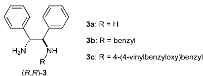
CHART 1. Chiral 1,2-Diamine Ligand
