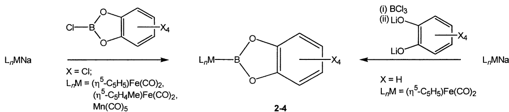
Scheme 1. Synthetic routes to boryl complexes 2–4 [ \text{L}_n\text{M}=(\eta^5\text{-C}_5\text{H}_5)\text{Fe}(\text{CO})_2 , \text{X}=\text{Cl} ( 2 ); \text{L}_n\text{M}=(\eta^5\text{-C}_5\text{H}_4\text{Me})\text{Fe}(\text{CO})_2 , \text{X}=\text{Cl} ( 2' ); \text{L}_n\text{M}=(\text{OC})_5\text{Mn} , \text{X}=\text{Cl} ( 3 ); \text{L}_n\text{M}=(\eta^5\text{-C}_5\text{H}_5)\text{Fe}(\text{CO})_2 , \text{X}=\text{H} ( 4 )].
