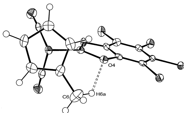
Fig. 2. Intramolecular C–H...O hydrogen bond between the methyl C–H and catecholboryl oxygen O(4) in 2' . Relevant bond lengths (Å) and angles (°): C(6)···O(4) 3.279(7), H(6a)···O(4) 2.52, C(6)–H(6a) 0.98, C–H...O 134.4.
