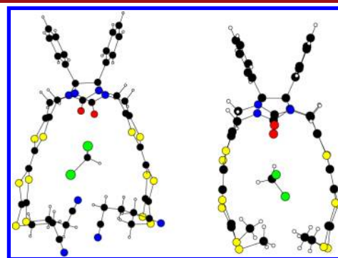
Figure 2. X-ray crystallographic structures of molecular clips 2 (left) and 3 (right).
