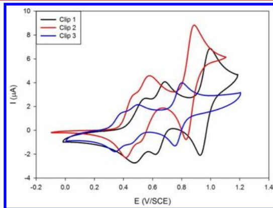
Figure 3. Cyclic voltammograms of molecular clips 1 (dark), 2 (red), and 3 (blue) in \text{CH}_2\text{Cl}_2/\text{CH}_3\text{CN} 3:1 recorded in n\text{-Bu}_4\text{NPF}_6 0.1 M solution as the supporting electrolyte, with platinum wires as counter and working electrodes.
