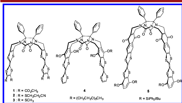
Figure 1. Formula of glycoluril-TTF molecular clips.
