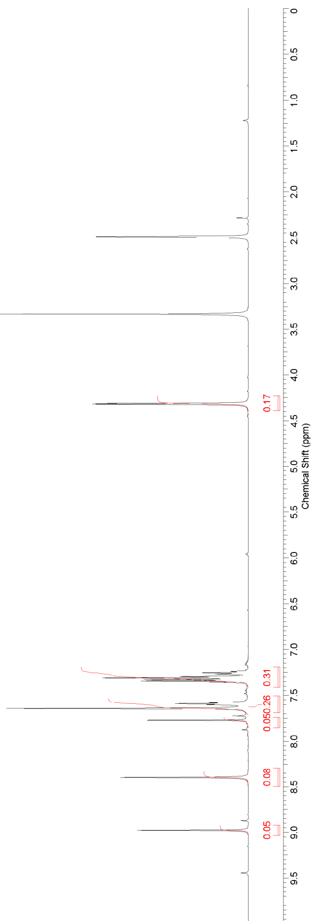
Spectrum 11. ^1\text{H} NMR of compd 10d (500 MHz, \text{DMSO-d}_6 ).
