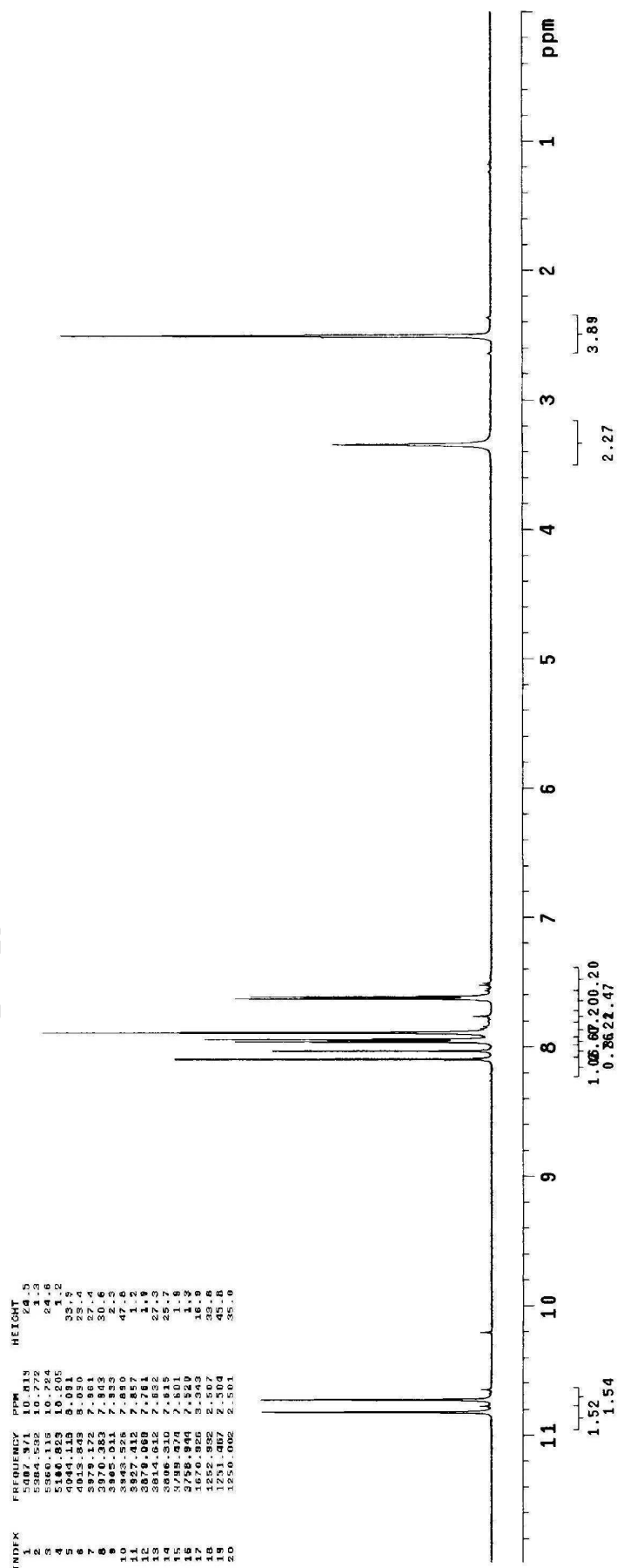
Spectrum 3. ^1\text{H} NMR of compd 6c (500 MHz, \text{DMSO-d}_6 ).
