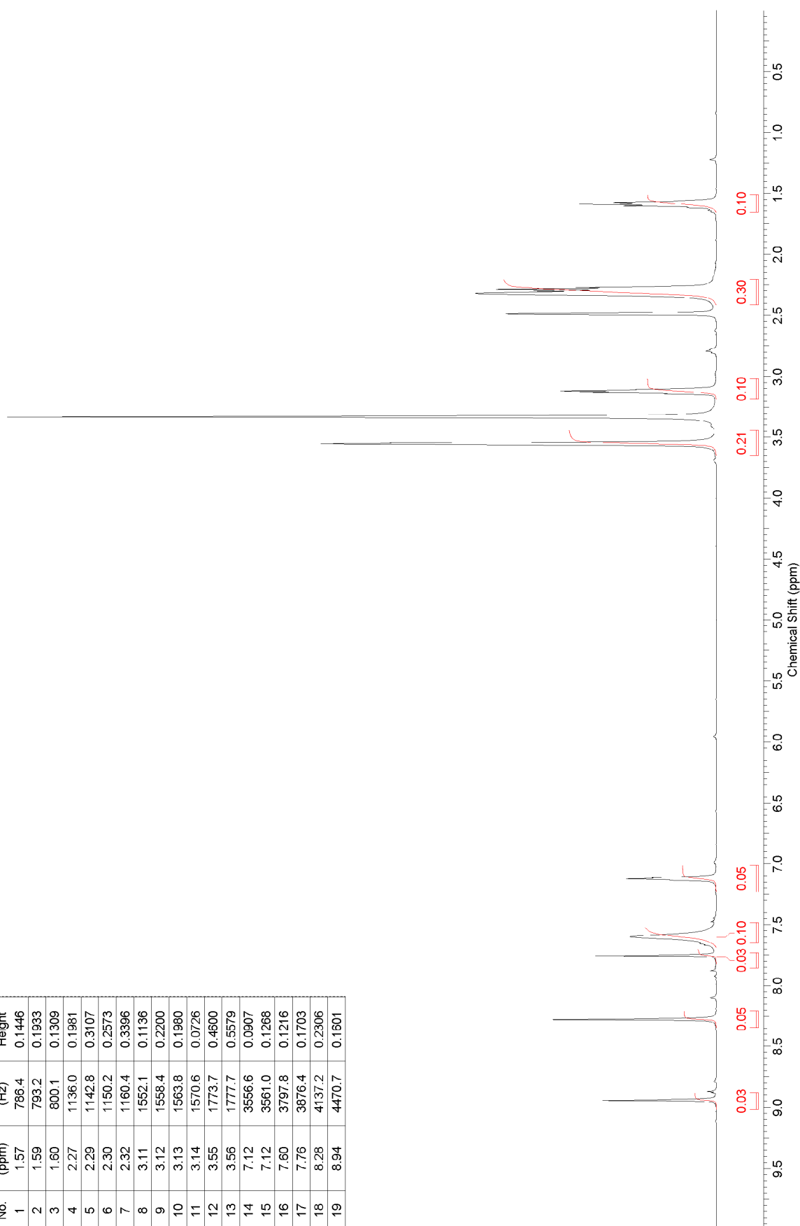
Spectrum 14. ^1\text{H} NMR of compd 10h (500 MHz, \text{DMSO-d}_6 ).
