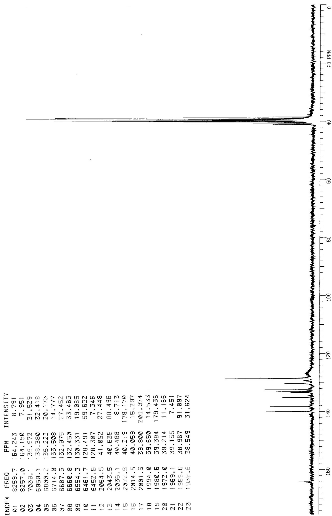
Spectrum 2. 13 C NMR of compd 5b (50 MHz, DMSO-d 6 ).
