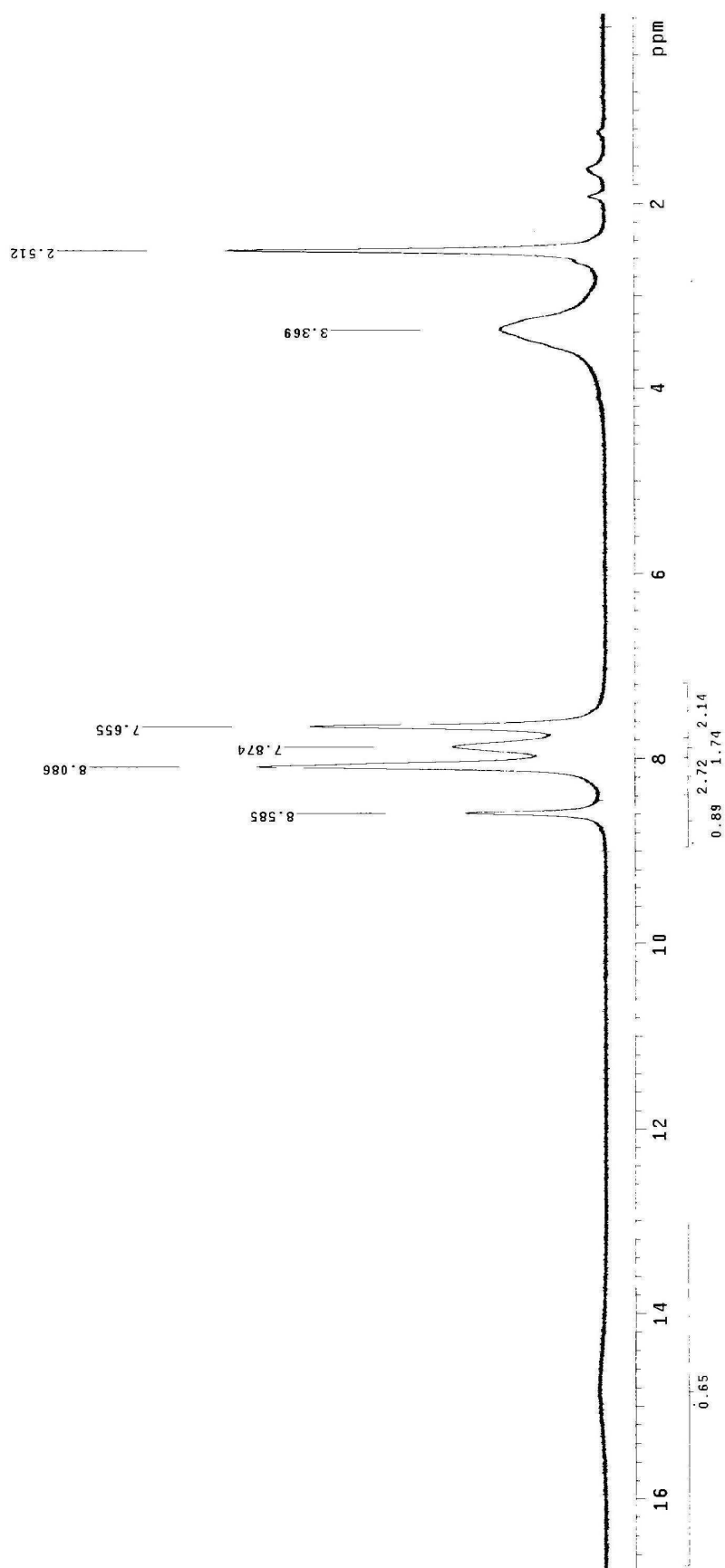
Spectrum 4. 1 H NMR of compd 7d (500 MHz, DMSO-d 6 ).
