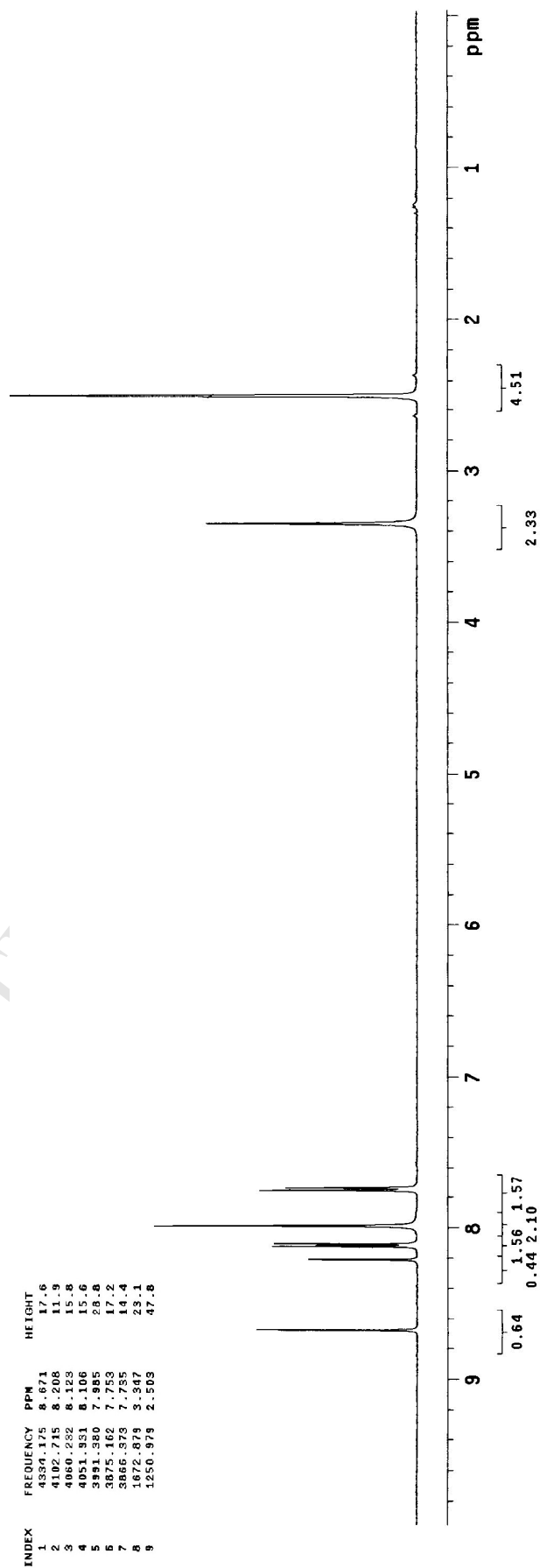
Spectrum 8. ^1\text{H} NMR of compd 7h (500 MHz, DMSO- \text{d}_6 ).
