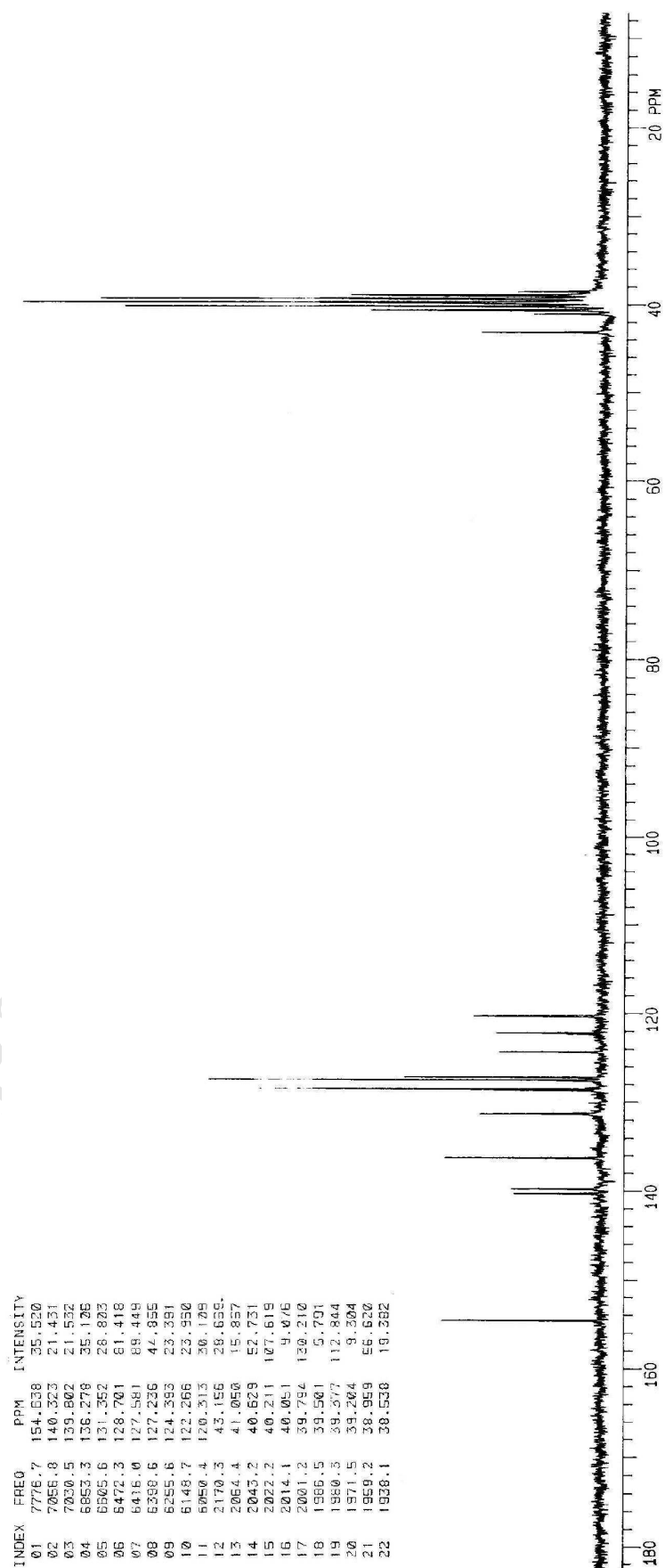
Spectrum 12. ^{13}\text{C} NMR of compd 10d (50 MHz, \text{DMSO-d}_6 ).
