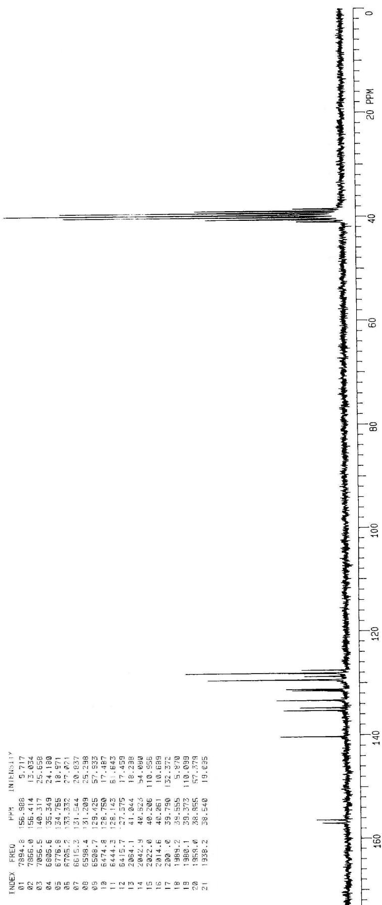
Spectrum 5. 13 C NMR of compd 7d (50 MHz, DMSO-d 6 ).
