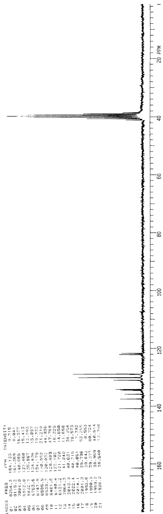
Spectrum 9. 13 C NMR of compd 7h (50 MHz, DMSO-d 6 ).
