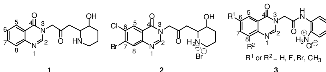
Fig. 1. Structures of compounds 1-3
