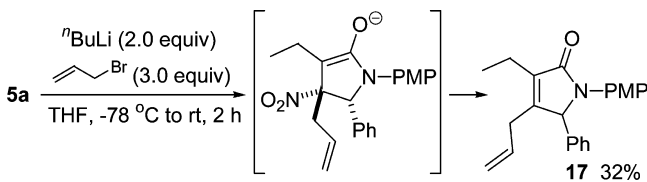
Scheme 7. Attempted \alpha -Functionalization
