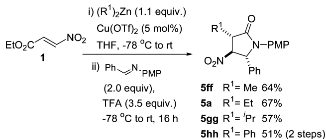
Scheme 4. Use of Common Di-organo Zinc Nucleophiles
