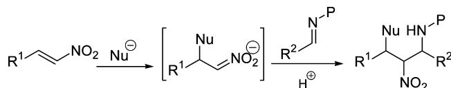
Scheme 1. Conjugate Addition Nitro-Mannich Reaction
