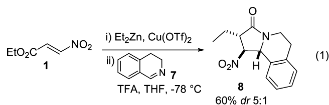
Scheme 4. Use of Common Di-organo Zinc Nucleophiles
