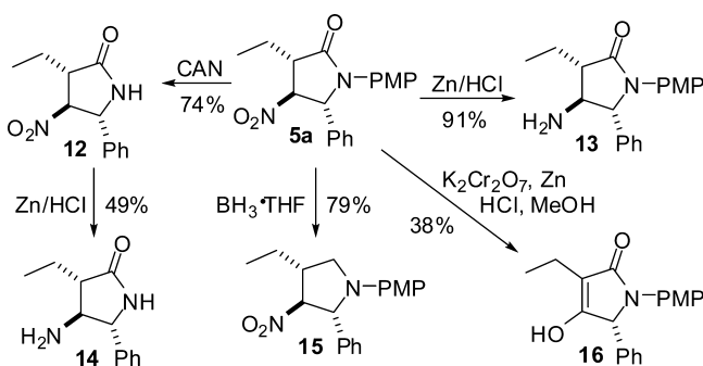
Scheme 6. Chemoselective Functional Group Interconversions
