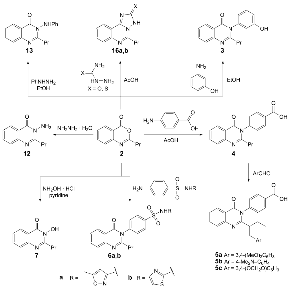
Scheme 2
