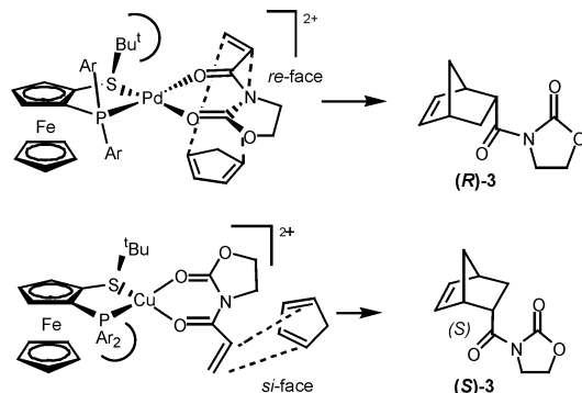
Figure 4. Proposed models for the ADA reaction.
