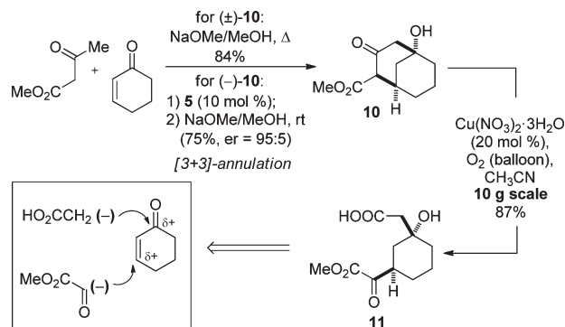
Scheme 4. Formal Conjugate Glyoxylation/Ketone Acetate Aldolization Sequence
