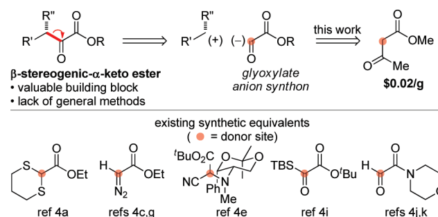
Figure 1. Synthetic equivalents for the glyoxylate anion synthon.
