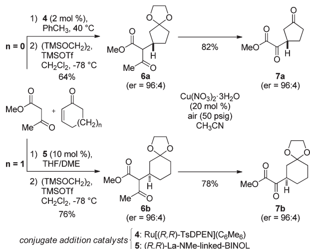
Scheme 2. Formal Conjugate Glyoxylation of Cyclic Enones
