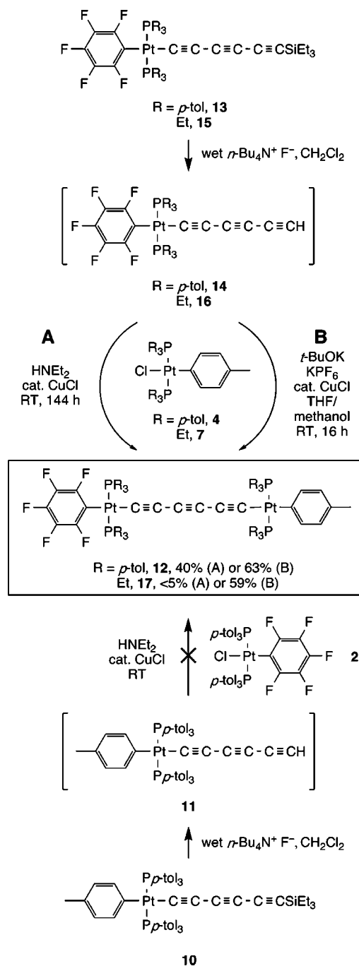
Scheme 4. Syntheses of Unsymmetrically Substituted Diplatinum Hexatriynediyl Complexes
