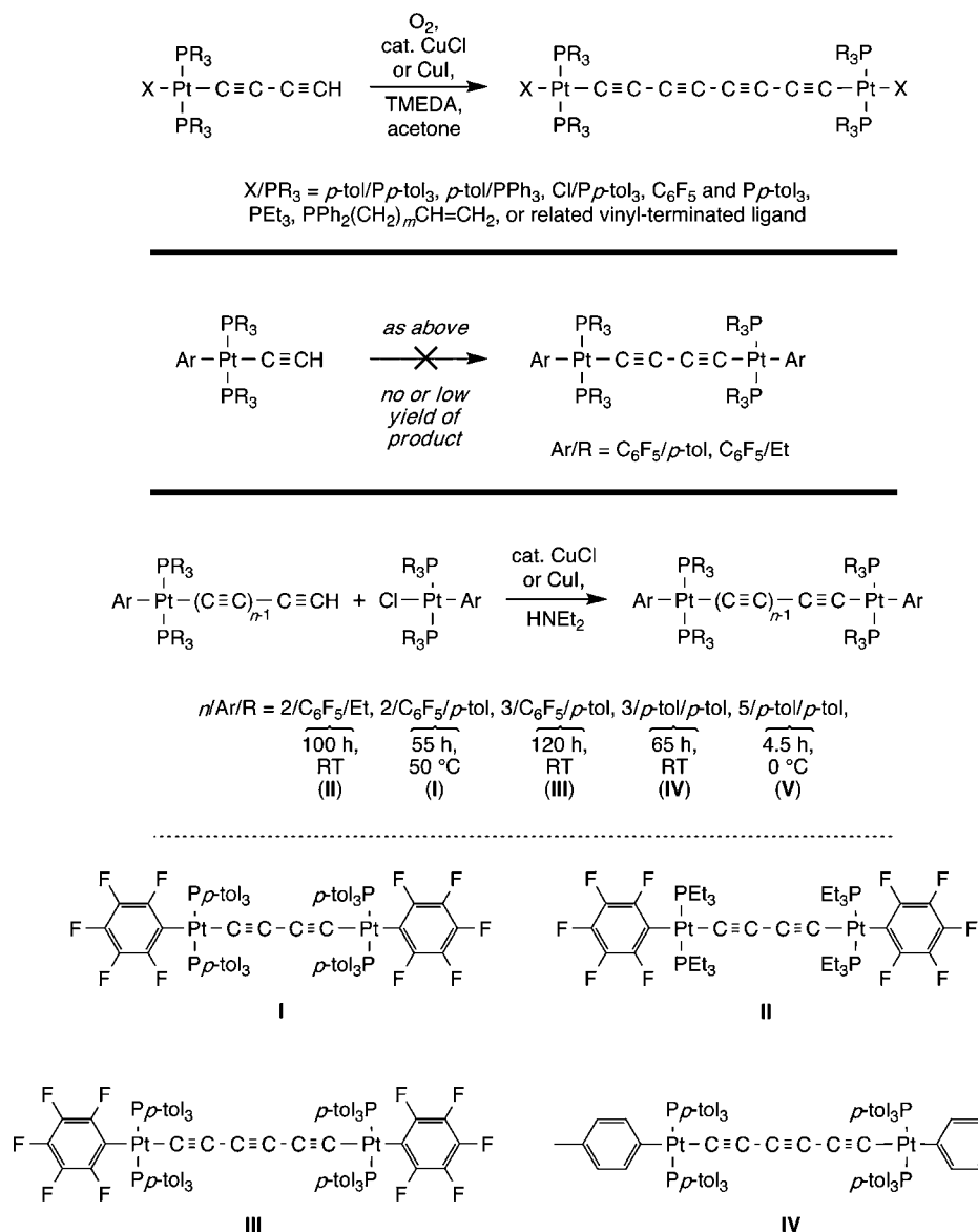
Scheme 1. Previously Investigated Coupling Routes to Symmetrically Substituted Diplatinum Polyynediyl Complexes
