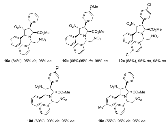
Figure 2. Compounds 10 isolated and characterized.
