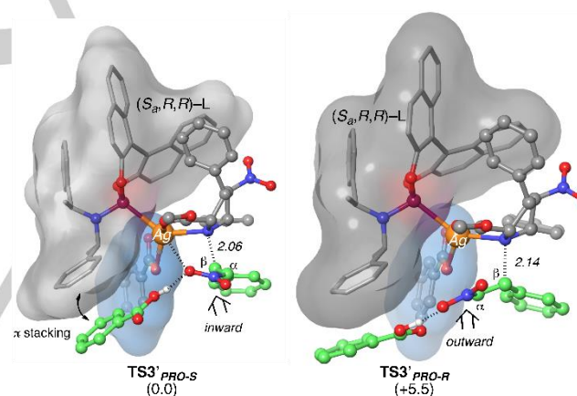
Figure 3. Main geometrical features and relative Gibbs Free energies of transition structures associated with the Michael addition step in presence of benzoic acid as additive computed at M06(PCM)/6-311+G**&LANL2DZ// ONIOM(B3LYP/6-31G*&LANL2DZ:UFF) level. Second molecule of \beta -nitrostyrene and the additive are highlighted in green. Relative Gibbs free energies and distances are in kcal·mol -1 and Å respectively.
