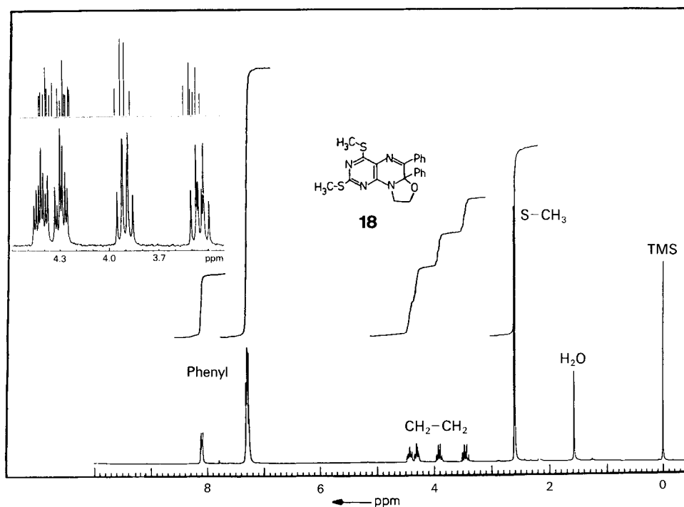
Fig. 1. 1 H-NMR spectrum (CDCl 3 ) of 18
