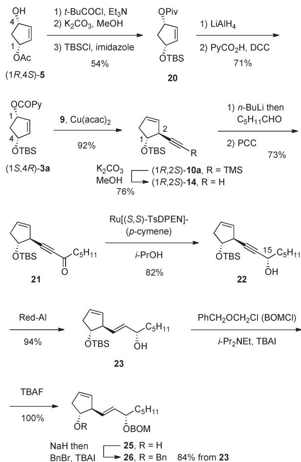
Scheme 3. Synthesis of the PGF 2α Intermediate
