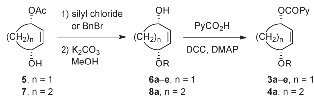
Scheme 1. Synthesis of Allylic Substrates 3a–e and 4a a
