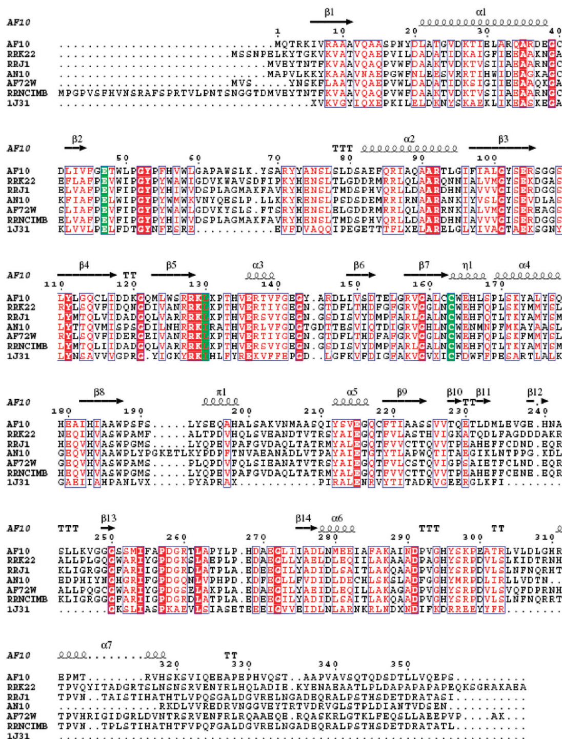
Figure 1. Structure-based alignment of nitrilase from different origins. AF10, an arylacetone nitrilase from A. faecalis ZJUTB10; RRK22, an aliphatic nitrilase from Rhodococcus rhodochrous K22 (D12583); RRJ1, an aromatic nitrilase from R. rhodochrous J1 (D11425); AN10, an aromatic nitrilase from Aspergillus niger K10 (EU282000); RRNCIMB, an aromatic nitrilase from R. rhodochrous NCIMB 11216 (CAC88237); 72W, an aliphatic nitrilase from Acidovorax facilis 72W (DQ444267); 1J31, hypothetical protein PH0642 (PDB accession code 1J31) one of the templates. The red color indicates the conserved catalytic residues: The residues influencing the triad pocket (Cys-163, Glu-47, and Lys-129) are marked in green.
