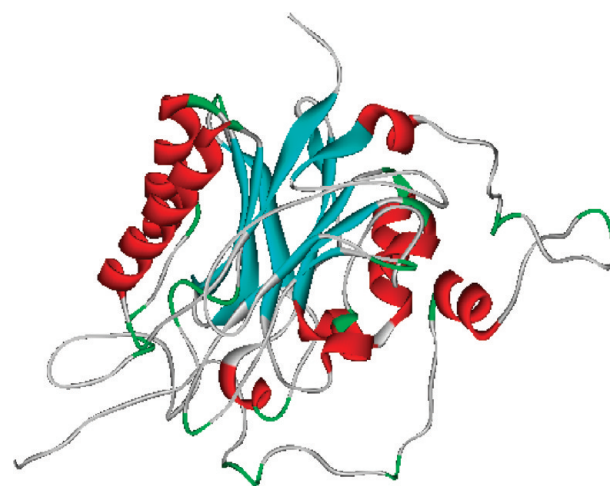
Figure 8. View of modeled structure of A. faecalis ZJUTB10 nitrilase.
