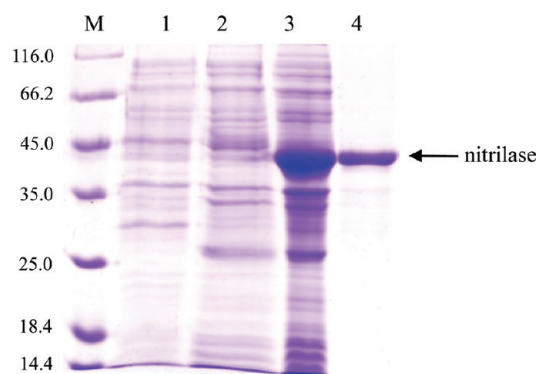
Figure 2. SDS-PAGE analysis of expression products by E. coli BL21-DE3 (pET-28b(+)-NIT). Gels with 30% polyacrylamide were subjected to protein analysis, and the protein bands were stained with Coomassie blue R250. M: Protein marker \beta -galactosidase (116.0 kDa), bovine serum albumin (66.2 kDa), ovalbumin (45 kDa), lactate dehydrogenase (35.0 kDa), REase Bsp98I (20.1 kDa), \beta -lactoglobulin (18.4 kDa), and lysozyme (14.4 kDa). Lanes 1 and 2 stand for the products of E. coli BL21 (DE3) control and E. coli BL21 (DE3) [pET-28b(+)-NIT] negative, lane 3 stands for induced E. coli BL21 (DE3) [pET28b(+)-NIT], and lane 4 stands for purified nitrilase.
