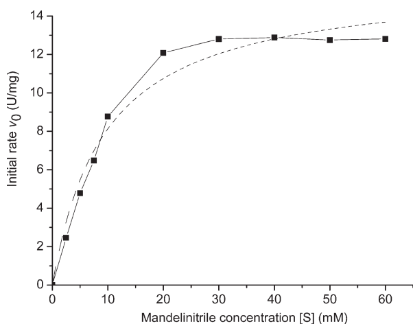
Figure 7. Reaction rate at different mandelonitrile concentrations. Reactions were performed for 10 min at 40 °C, 150 rpm, with 50 mM Tris-HCl buffer (pH 7.5): (···) fitting curve, (—) experimental curve.
