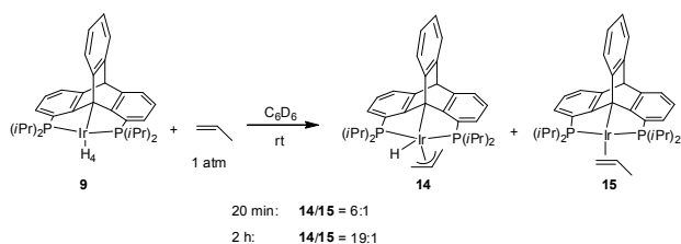
Scheme 4. Formation of \text{Ir}(\eta^3\text{-propenyl})(\text{H}) 14 and \text{Ir}(\eta^2\text{-propene}) 15
