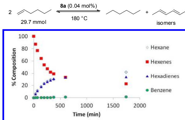
Figure 4. Product distribution after 29 h from disproportionation of 1-hexene with 8a .
