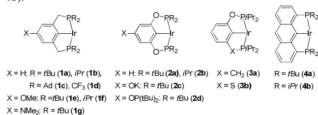
Figure 1. Examples of active PCP iridium pincer complexes for alkane dehydrogenation.
