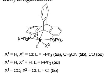
Figure 2. Iridium triptycene-based pincer complexes developed by Gelman.
