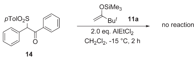
Scheme 8 Attempt to use a \beta -ketosulfone bearing a simple phenyl group in the Lewis acid promoted substitution reaction.
