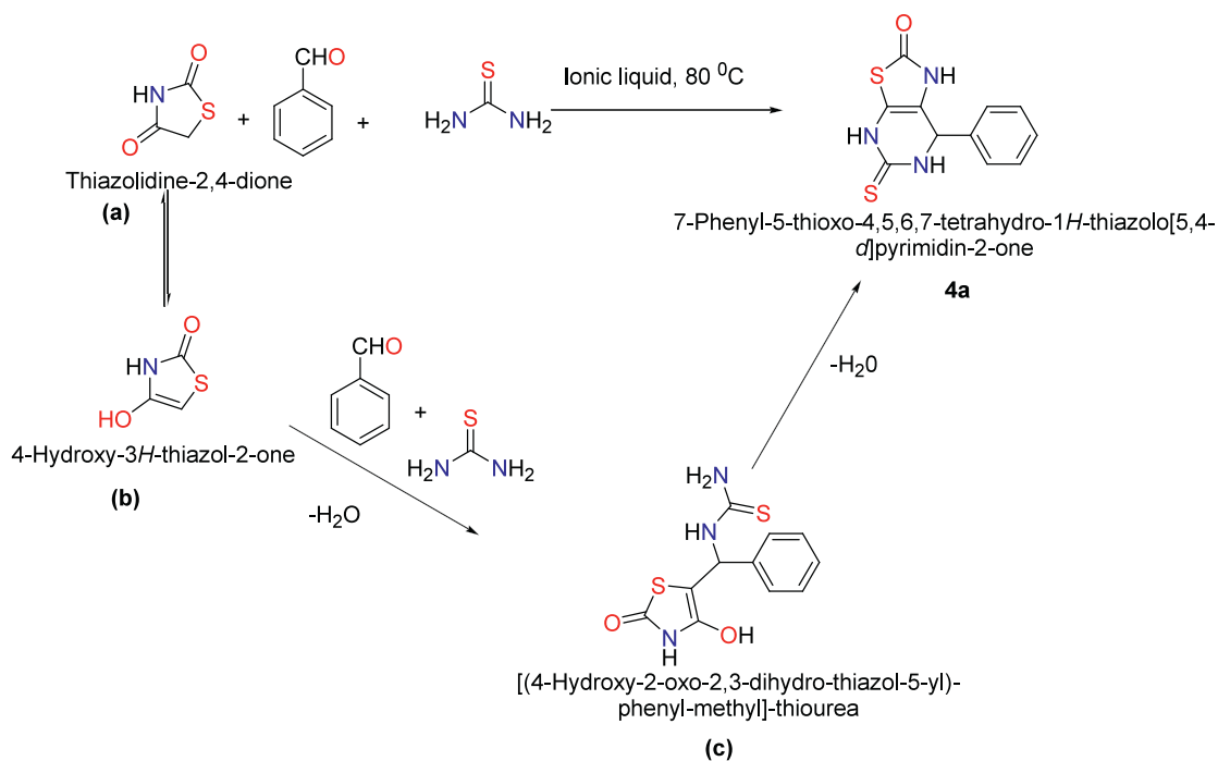
Scheme 1. Mechanism for the synthesis of 7-phenyl-1,4,6,7-tetrahydro-thiazolo[5,4- d ]pyrimidine-2,5-diones.
