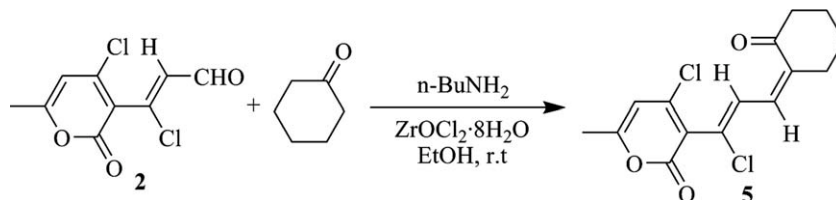
Scheme 5. Aldol reaction of 2 with cyclohexanone in the presence of n -BuNH 2 /ZrOCl 2 ·8H 2 O.
