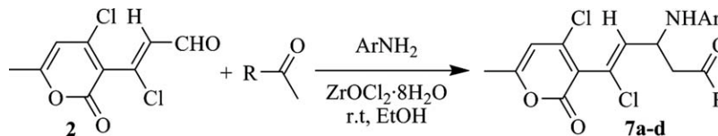
Scheme 6. Mannich reaction of 2 , anilines and acyclic ketones.
