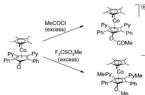
Scheme 2. Acetylation and complete methylation of [\text{Cp}^*\text{Co}(\eta^4\text{-1})] . Py = 2-pyridyl.
