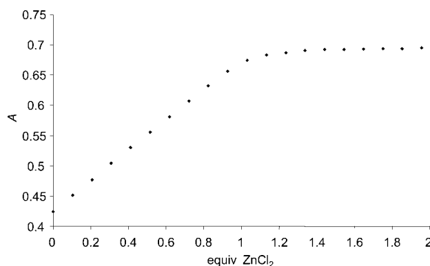
Figure 9. Absorbance at \lambda = 297 \text{ nm} during the titration of 1 with zinc chloride (portionwise addition of 2 equiv) in acetonitrile.
