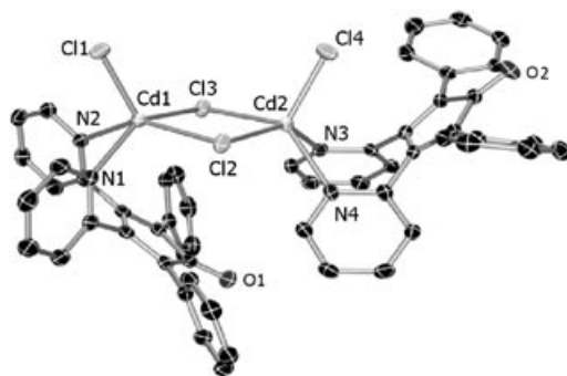
Figure 6. Molecular structure of [(1)\text{Cd}(\mu\text{-Cl})\text{Cl}]_2 in the crystal.
