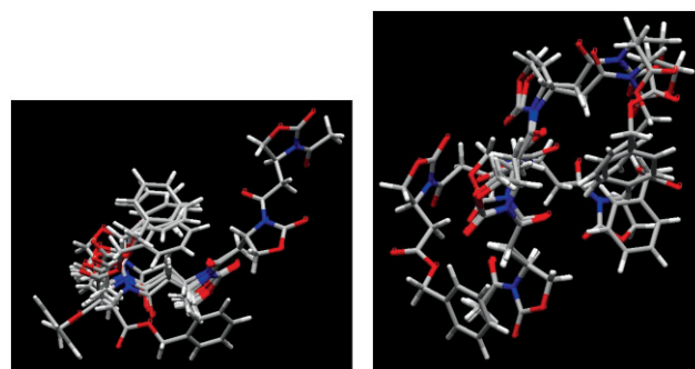
Fig. 4 Superposition of the six most stable conformations for Ac-(D-Oxac) 4 -OBn in water (left) and in chloroform (right). The conformers were superimposed with “RMS Fit”, which allows to overlay two or more molecules by minimizing the distance between corresponding atoms in the two target molecules.
