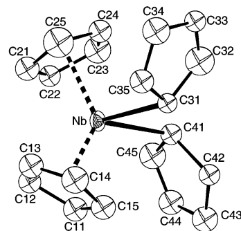
Fig. 1. View of the molecular structure of \text{NbCp}_4 .
