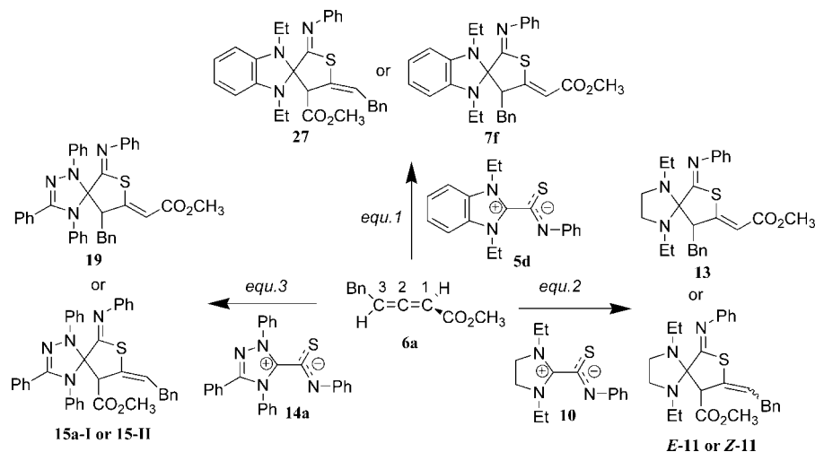
SCHEME 7. Computational Reactions of 2-Arylthiocarbamoyl Benzimidazolium 5d , -imidazolinium 10 , and -triazolium Salt 14a with 4-Benzylallenecarboxylate 6a
