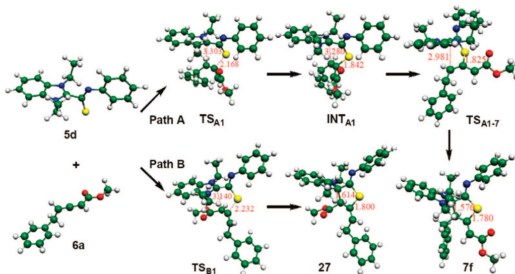
FIGURE 1. The obtained reaction pathways for 5d + 6a \rightarrow 7f and 5d + 6a \rightarrow 27 , along with the bond lengths (Å) for the main reaction coordinates.
