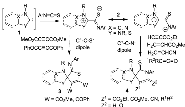
SCHEME 1. The Reactions between N -Heterocyclic Carbene-Derived Ambident Dipoles and Electron-Deficient Alkynes, Alkenes, and Ketenes
