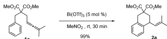
Scheme 1. \text{Bi}(\text{OTf})_3 -Catalyzed Transformation of 1a
