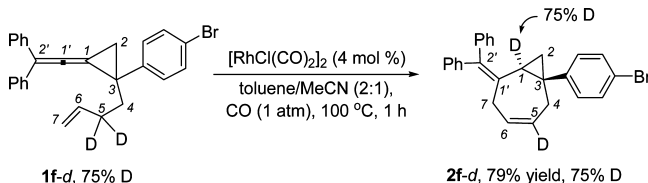
Scheme 3. Deuterium Labeling Study of Mechanism
