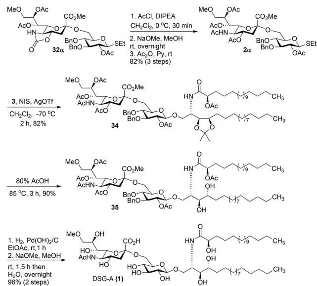
Scheme 7 Completion of the total synthesis of the ganglioside DSG-A (1).
