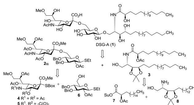
Scheme 1 Retrosynthesis of the ganglioside DSG-A (1).
