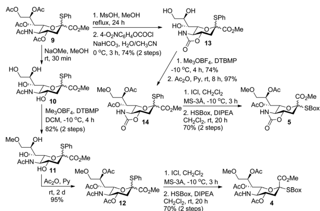
Scheme 2 Synthesis of the sialyl donors 4 and 5.
