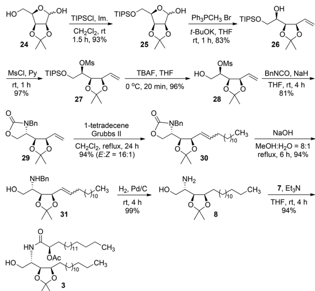
Scheme 5 Construction of the protected phytoceramide 3.
