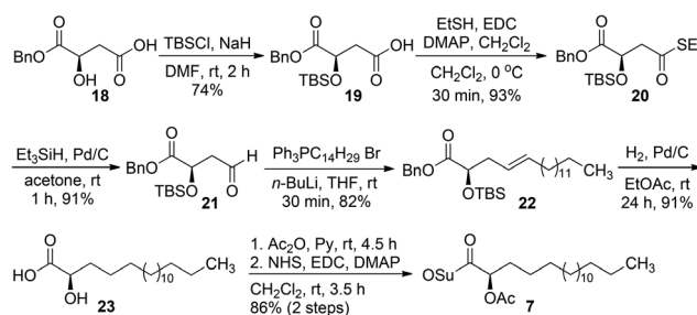
Scheme 4 Synthesis of the optically pure ( R )-2-hydroxyoctadecanoic acid derivative 7.
