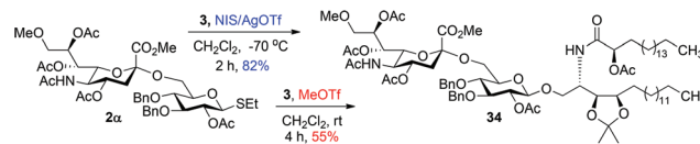
Scheme 6 Examination of the glycosylation of disaccharide 2α with phytoceramide 3 .
