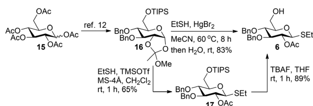
Scheme 3 Preparation of the glucose derivative 6.
