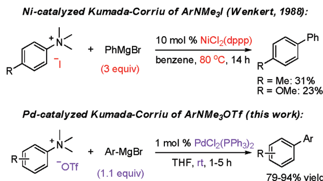
Scheme 1. Wenkert's Ni-Catalyzed Cross Coupling of Ar-NMe 3 I and Our Pd-Catalyzed Cross Coupling of Ar-NMe 3 OTf
