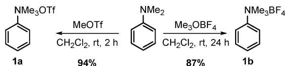
Scheme 2. Preparation of Triflate and Tetrafluoroborate Salts
