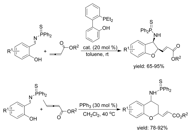
Scheme 1. Phosphine-Catalyzed Domino Reaction of Salicyl N -Thiophosphoryl Imines with Electron-Deficient Allenes
