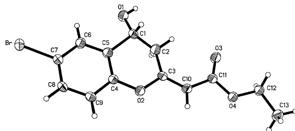
Figure 1. X-ray crystal structure of E-4c .
