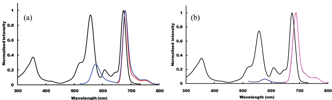
Figure 4. Normalized excitation spectrum (black, monitored at 750 nm) and fluorescence spectra (blue, \lambda_{\text{exc}} = 515 \text{ nm} and red, \lambda_{\text{exc}} = 640 \text{ nm} ) of 2 (a) and 3 (b) in \text{CH}_2\text{Cl}_2 ( \sim 1.0 \times 10^{-6} \text{ M} ). Note that the emissions from the Pc moiety of 2 and 3 excited at 515 and 640 nm coincide almost completely.
